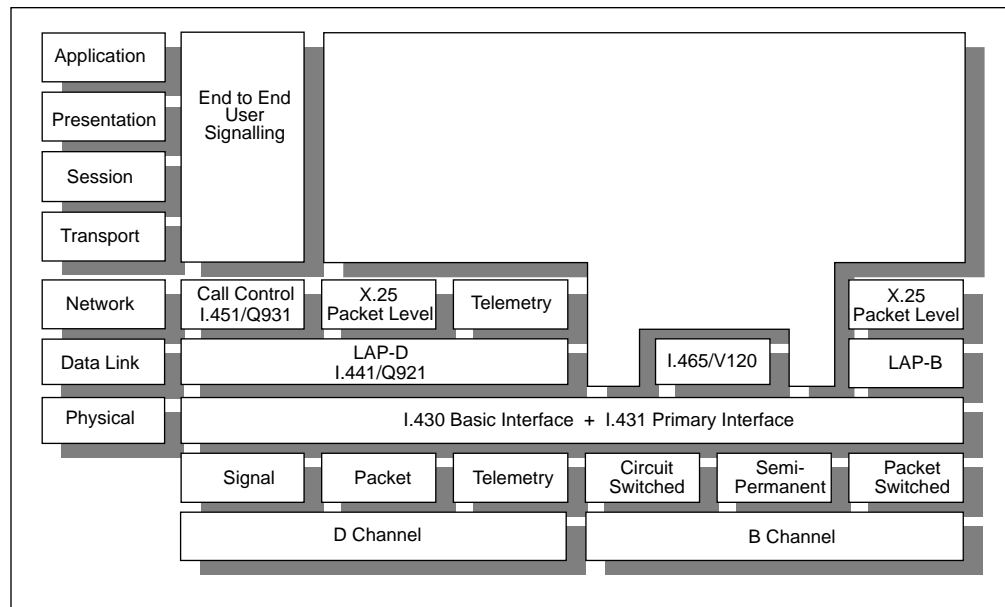
Figure 4-2 ISDN Protocol Architecture
