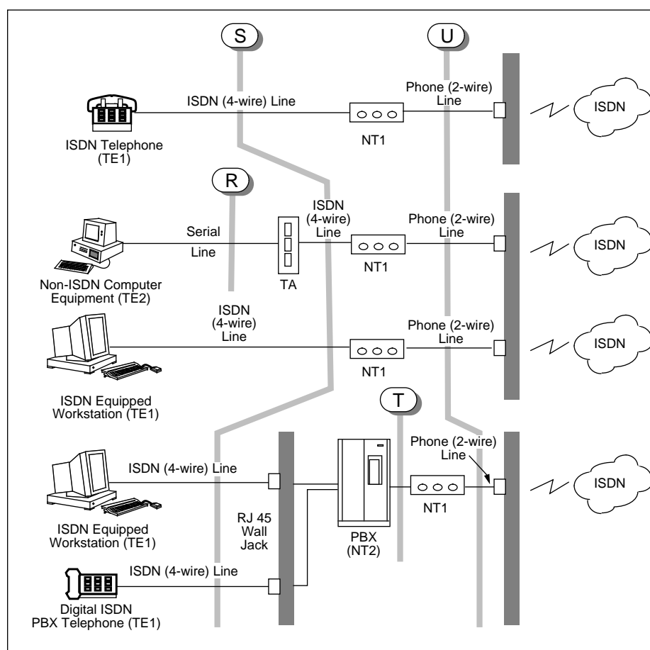
Figure 4-1 ISDN Reference Points
