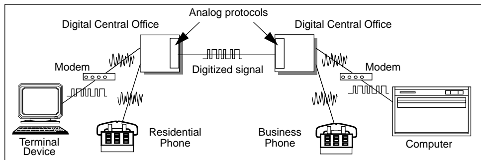
Figure 1-2 Digital and Analog Components of Most Telephone Systems Today
