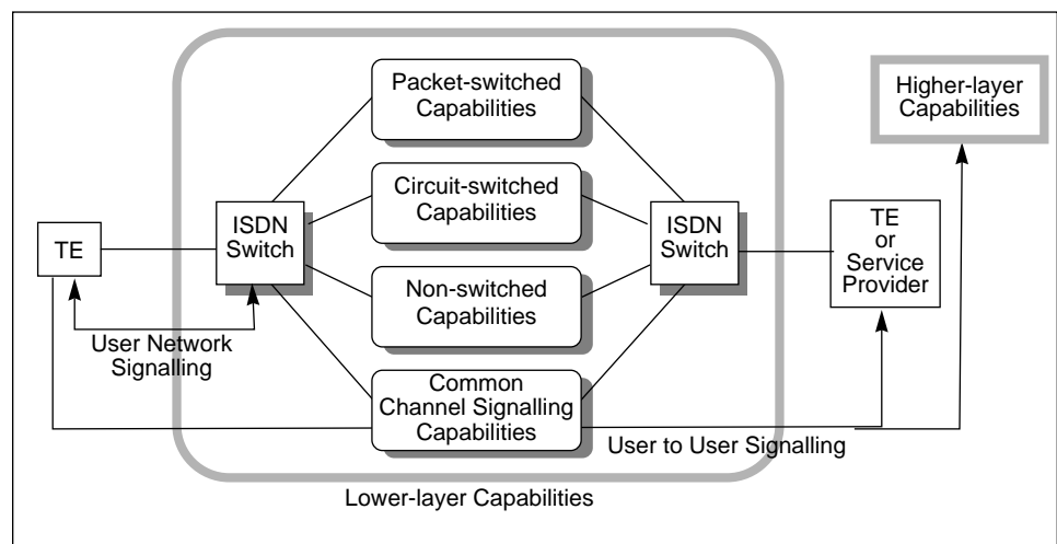
Figure 3-1 ISDN Architecture
