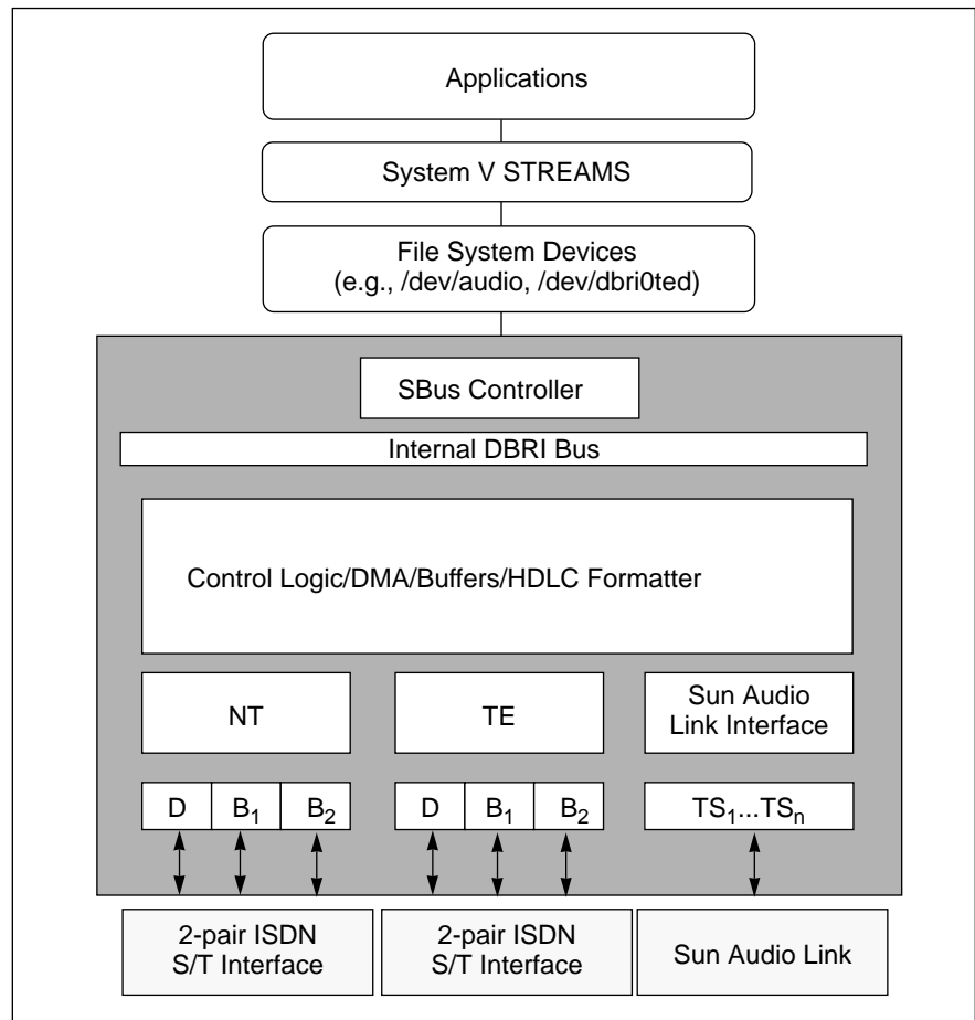
Figure 5-1 ISDN Dual Basic Rate Interface
