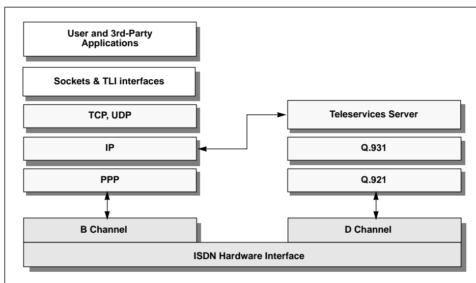
Figure 6-2 ISDN WAN Architecture
