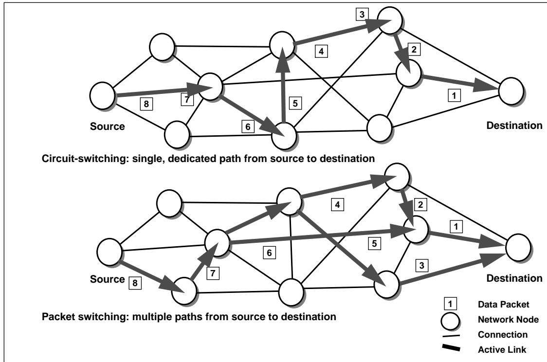
Figure 1-4 Circuit and Packet Switched Networks
