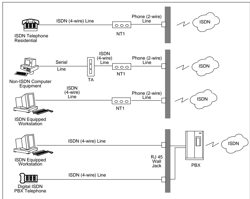
Figure 3-2 ISDN Connections
