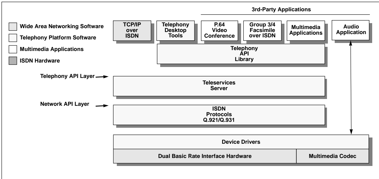
Figure 6-1 ISDN Software Architecture
