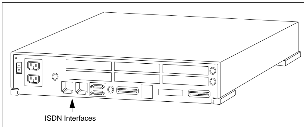
Figure 5-2 SPARCstation 10 ISDN Back Panel Connections
